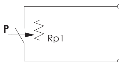
LINE BREAK DETECTION CIRCUIT
