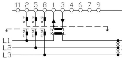
Connection -05
