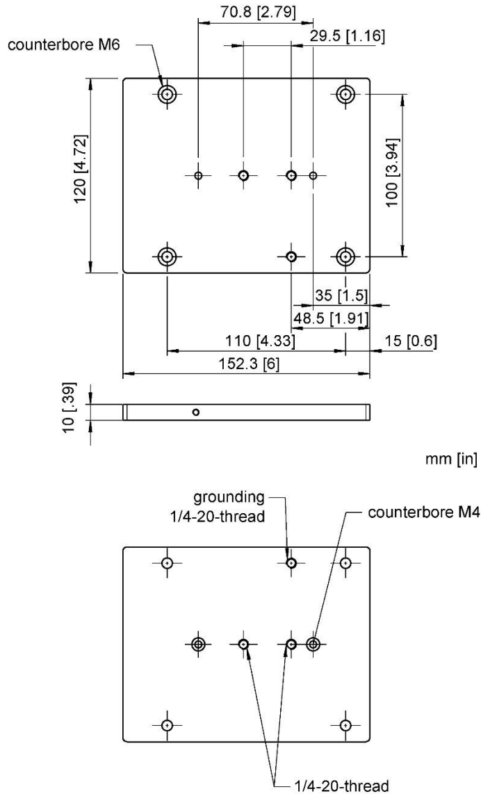
Figure 7-13: Mounting Base
