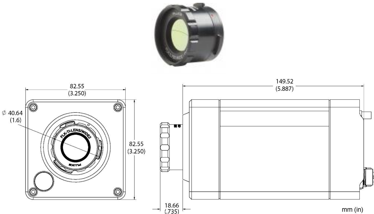
Figure 7-1: Wide Lens
